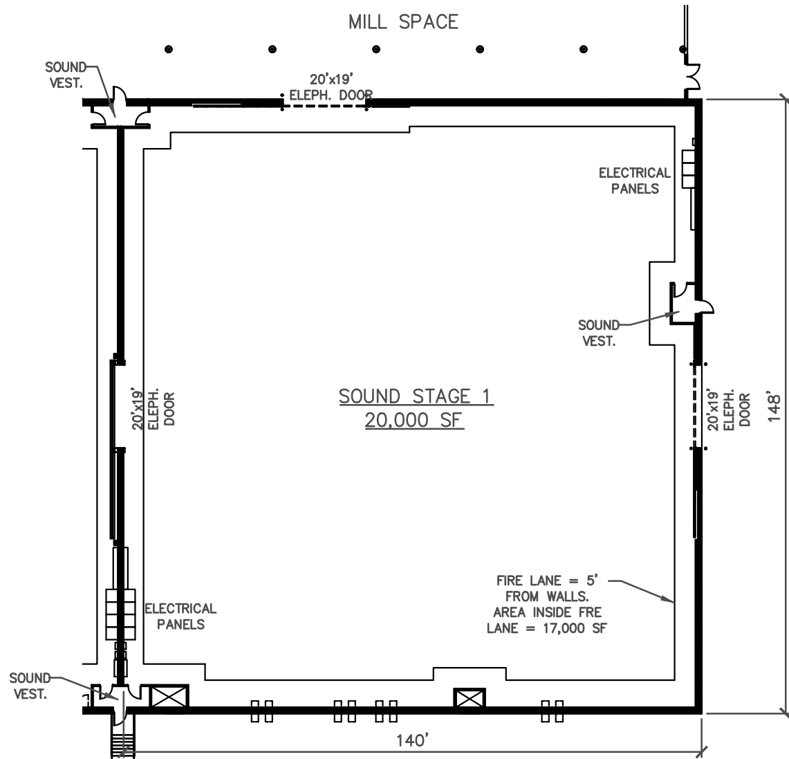
N ⊕ SOUND STAGE 1 SCALE: 1/32" = 1'-0"
