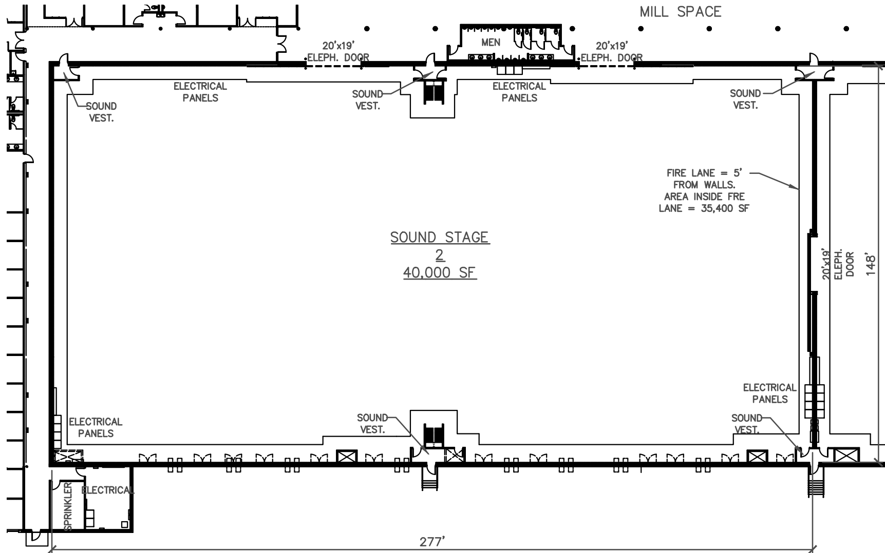
N ⊕ SOUND STAGE 2 SCALE: NONE
